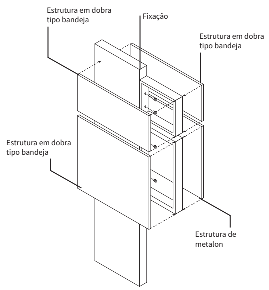
Vista explodida
